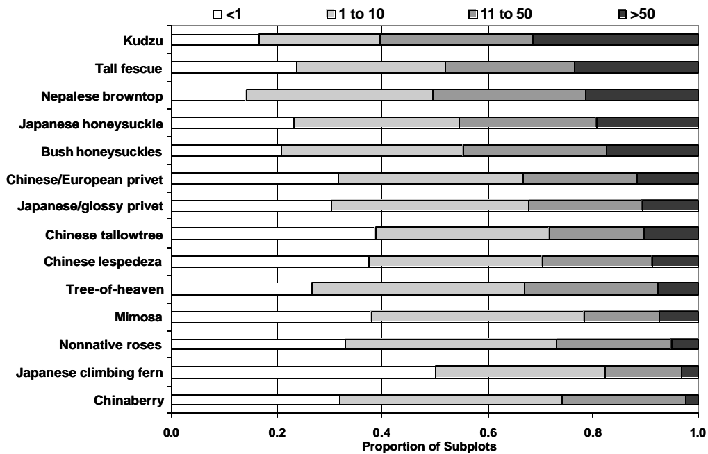
Figure 3.—Proportion of infested subplots by species and severity class (< 1, 1–10, 11–50, and >50 percent cover) for panels completed as of September 2004, southern United States.
