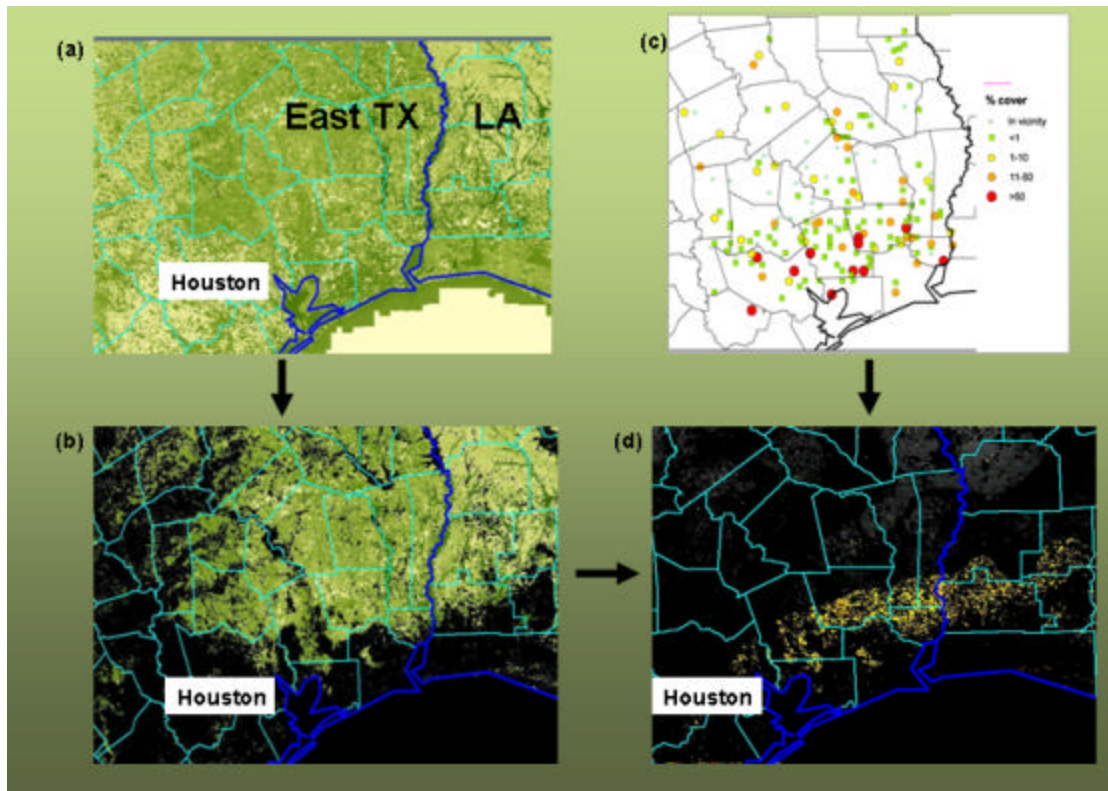
Figure 6.—Steps in the process of fine-scaled estimation of Chinese tallowtree biomass: (a) MODIS satellite imagery at 250-m resolution for east Texas and west Louisiana; (b) spectral value classification of forest and nonforest land; (c) Chinese tallowtree-infested FIA forest land sample locations in east Texas by presence and infestation severity (percent total cover); and (d) depiction of Chinese tallowtree biomass at 250-m resolution.
