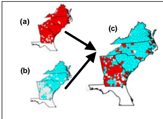
Figure 2.— Japanese honeysuckle distribution by county in Georgia, North Carolina, South Carolina, and Virginia: (a) FIA phase 2 field observations, 2001–04, (b) PLANTS Database 2002, largely from herbarium specimens, and (c) both combined: information from (b), with additions from (a).
