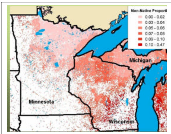
Figure 4.—Percent nonnative species on forest land by ecoregion, Michigan, Minnesota, and Wisconsin (Source: Olson et al. 2004).
